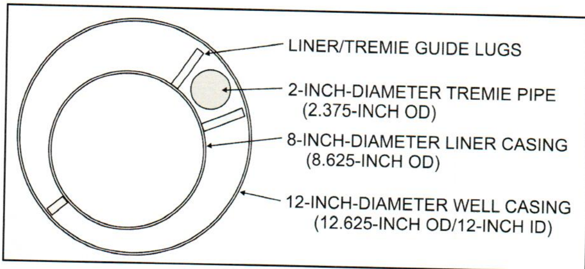
Figure 3 – Tremie and Liner Guide Lug Placement
