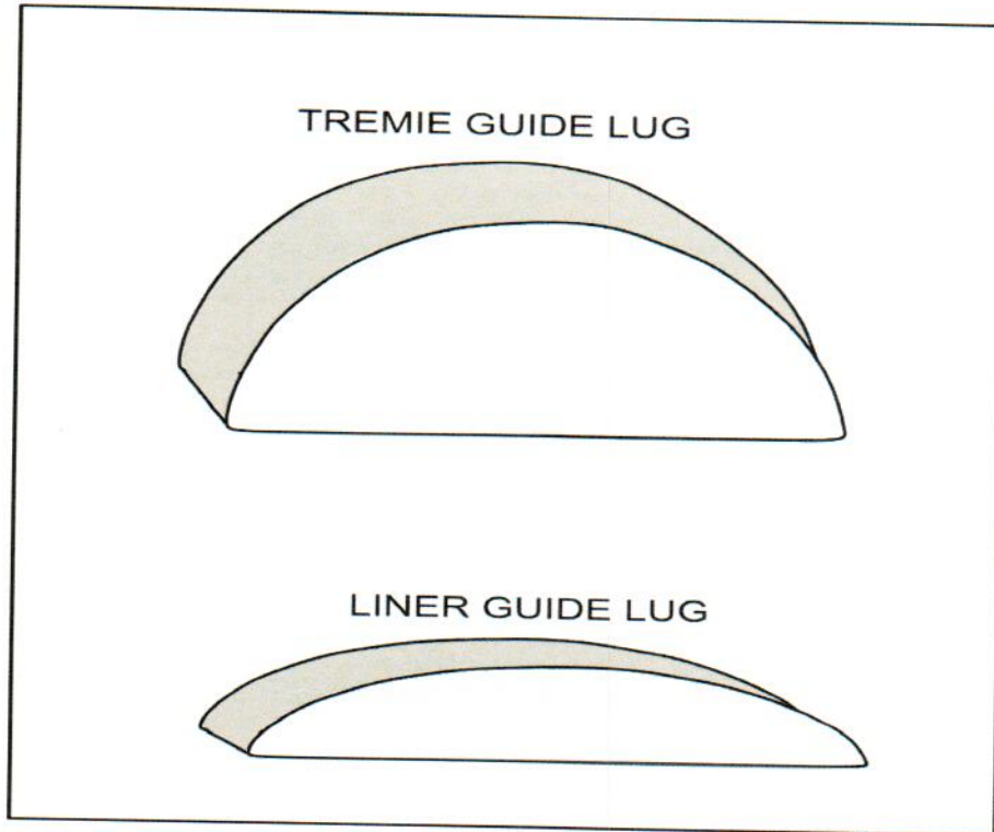
Figure 2 – Half Moon Tremie and Liner Guide Lugs
